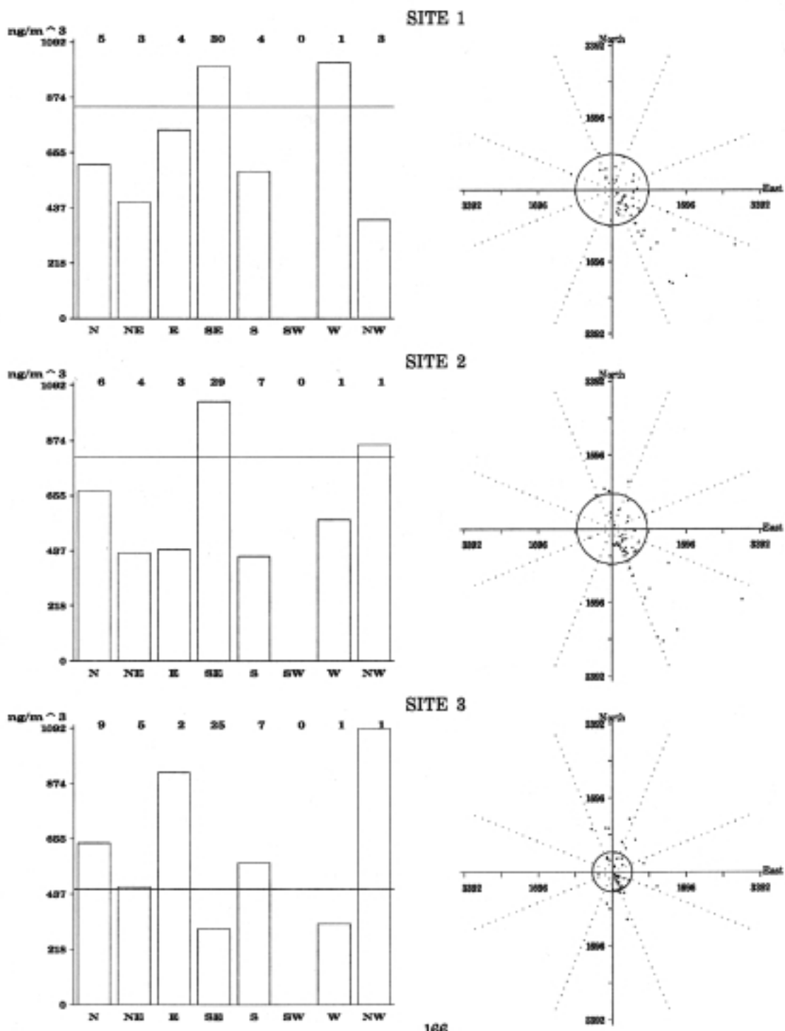
Figure 5.25. Bar charts and wind sector plots of coarse fraction Aluminum (Al) concentrations ( \text{ng}/\text{m}^3 ) at the three sites. See page 39 for a detailed explanation of figures.
