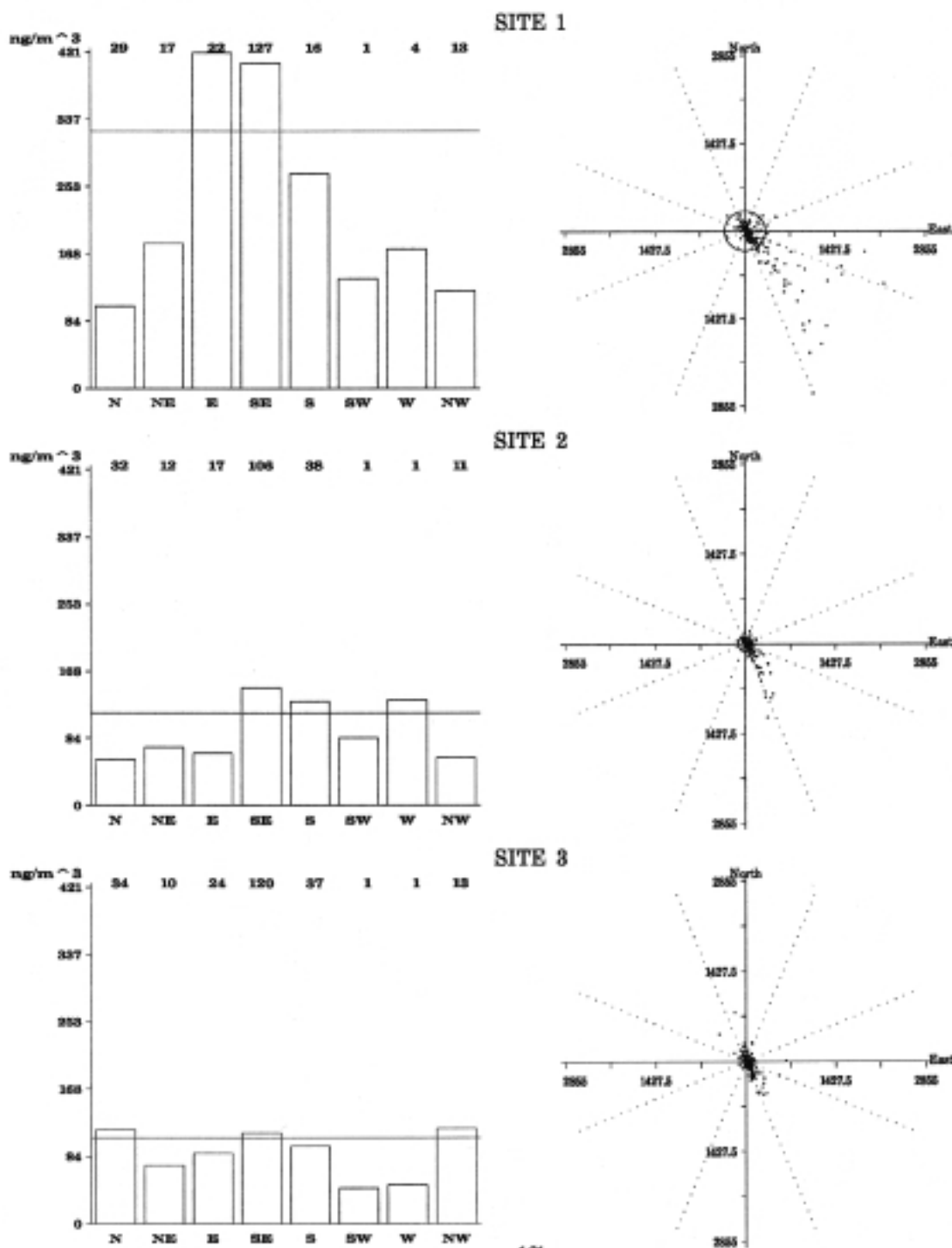
Figure 5.20. Bar charts and wind sector plots of fine fraction Silicon (Si) concentrations ( \text{ng}/\text{m}^3 ) at the three sites. See page 39 for a detailed explanation of figures.
