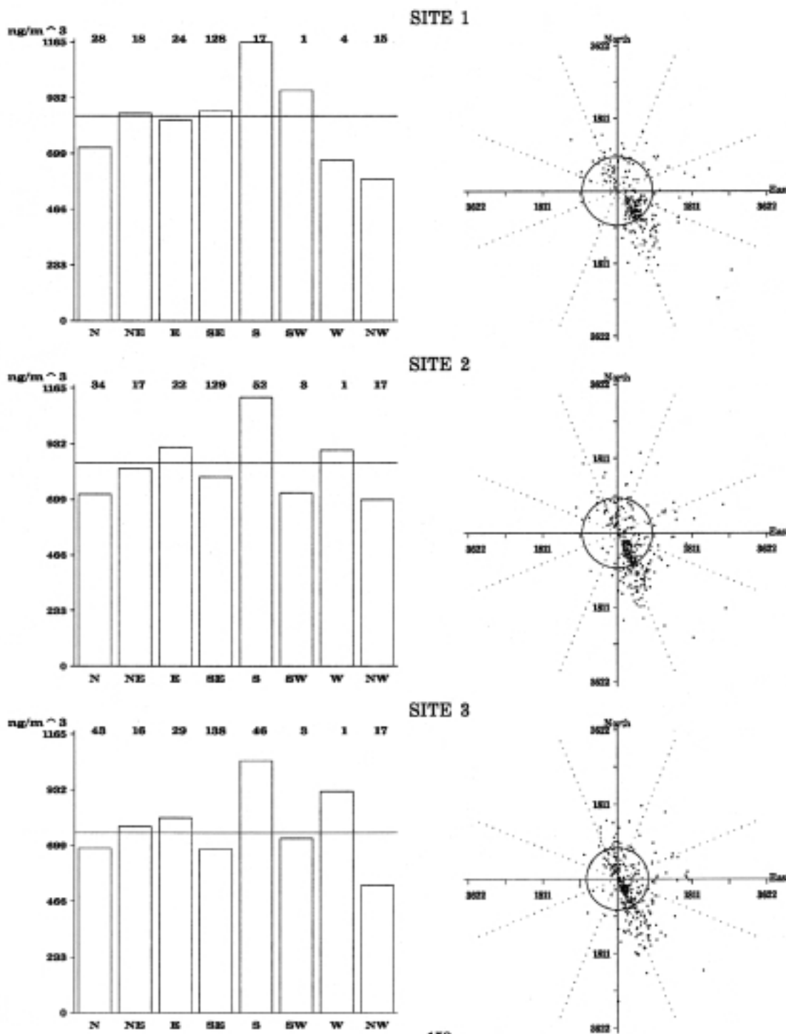
Figure 5.18. Bar charts and wind sector plots of fine fraction Sulfur (S) concentrations ( \text{ng}/\text{m}^3 ) at the three sites. See page 39 for a detailed explanation of figures.
