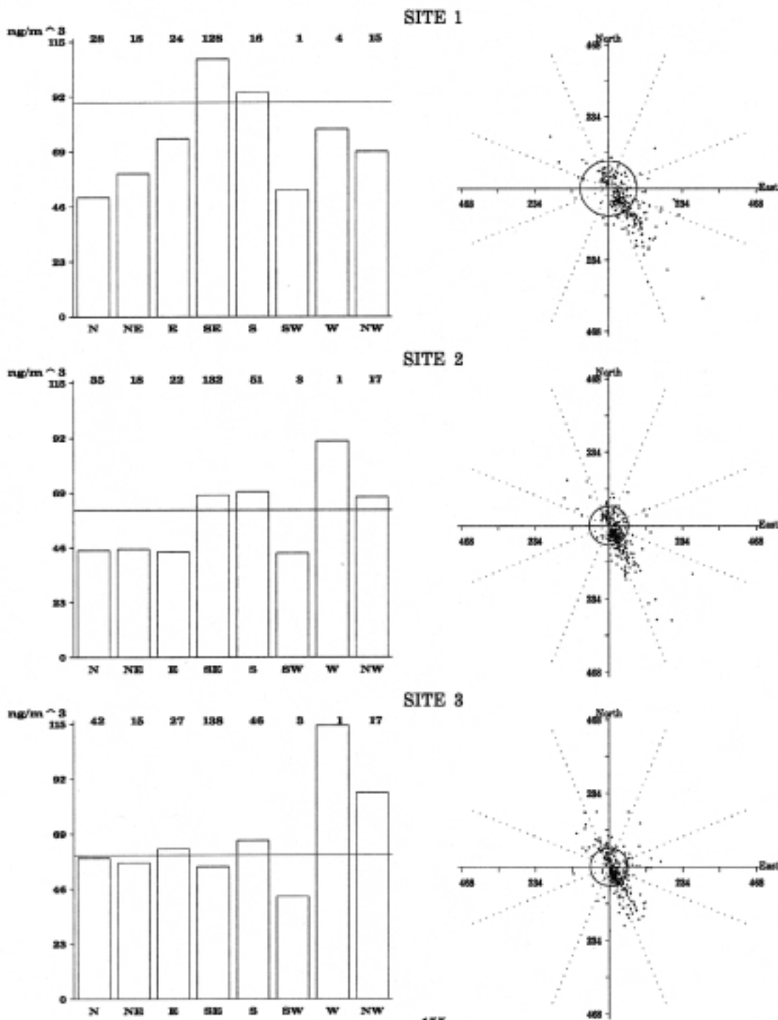
Figure 5.14. Bar charts and wind sector plots of fine fraction Potassium (K) concentrations ( \text{ng}/\text{m}^3 ) at the three sites. See page 39 for a detailed explanation of figures.
