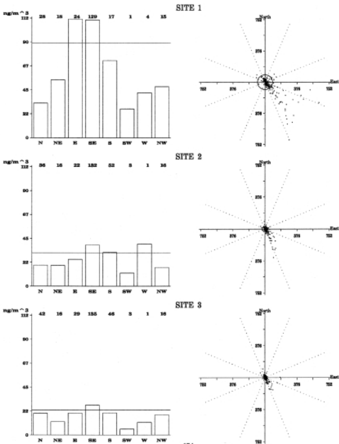
Figure 5.13. Bar charts and wind sector plots of fine fraction Iron (Fe) concentrations ( \text{ng}/\text{m}^3 ) at the three sites. See page 39 for a detailed explanation of figures.
