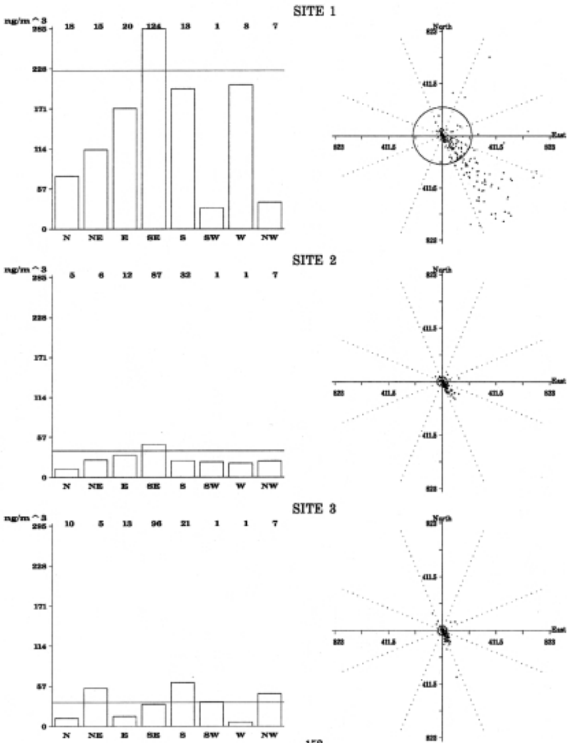
Figure 5.12. Bar charts and wind sector plots of fine fraction Chlorine (Cl) concentrations (ng/m 3 ) at the three sites. See page 39 for a detailed explanation of figures.
