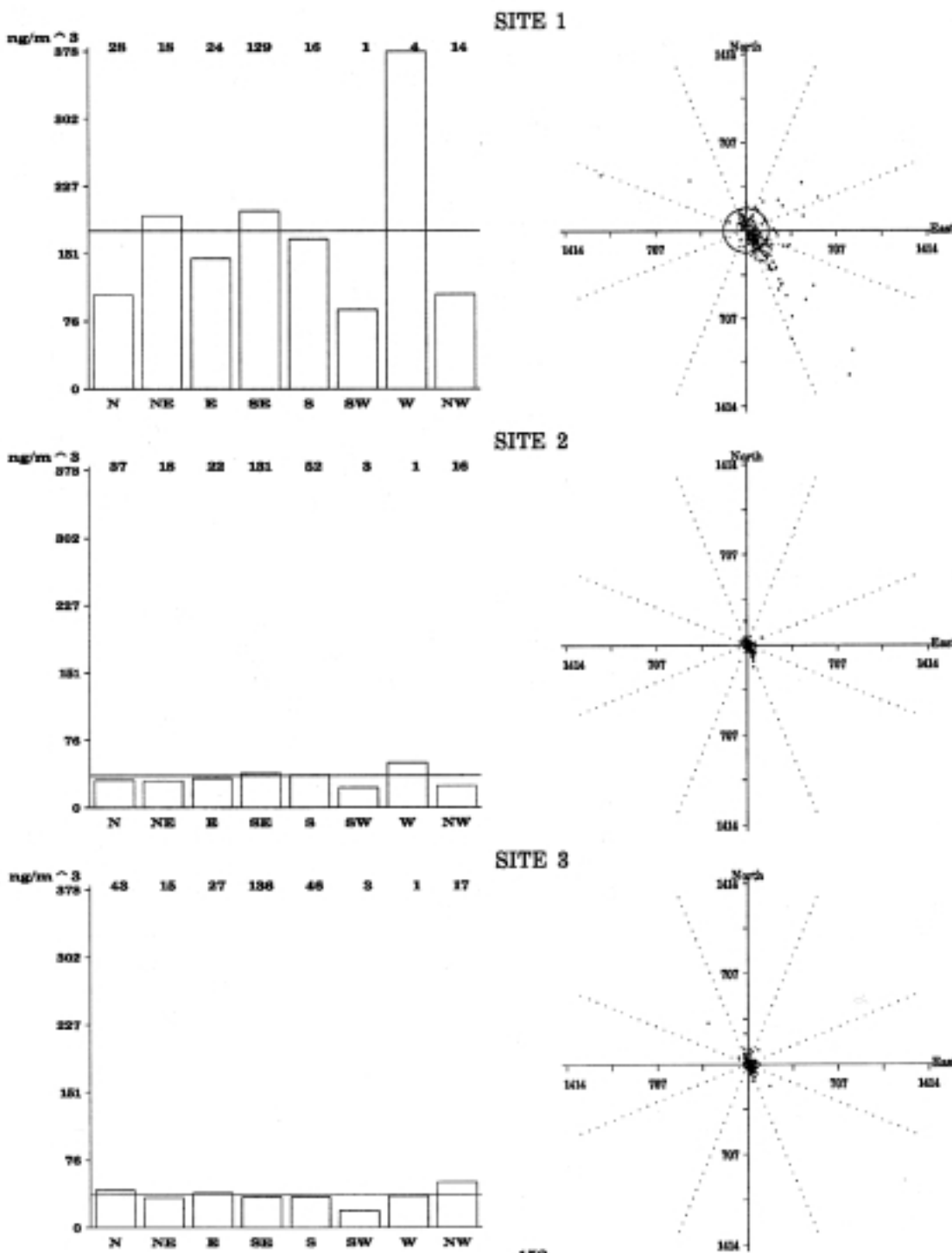
Figure 5.11. Bar charts and wind sector plots of fine fraction Calcium (Ca) concentrations ( \text{ng}/\text{m}^3 ) at the three sites. See page 39 for a detailed explanation of figures.
