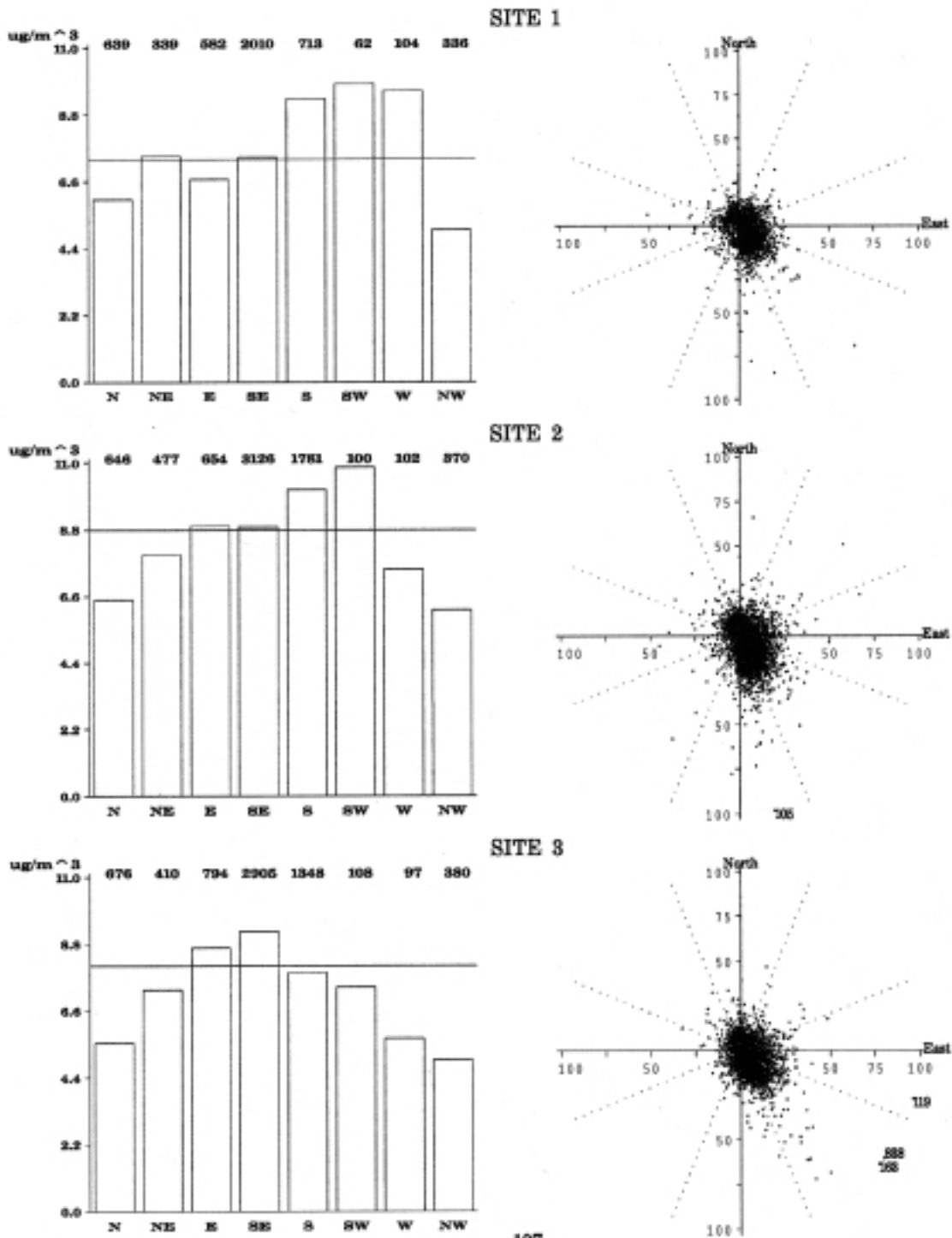
Figure 5.1. Bar charts and wind sector plots of hourly PM2.5 concentrations ( \mu\text{g}/\text{m}^3 ) at the three sites. See page 39 for a detailed explanation of figures.
