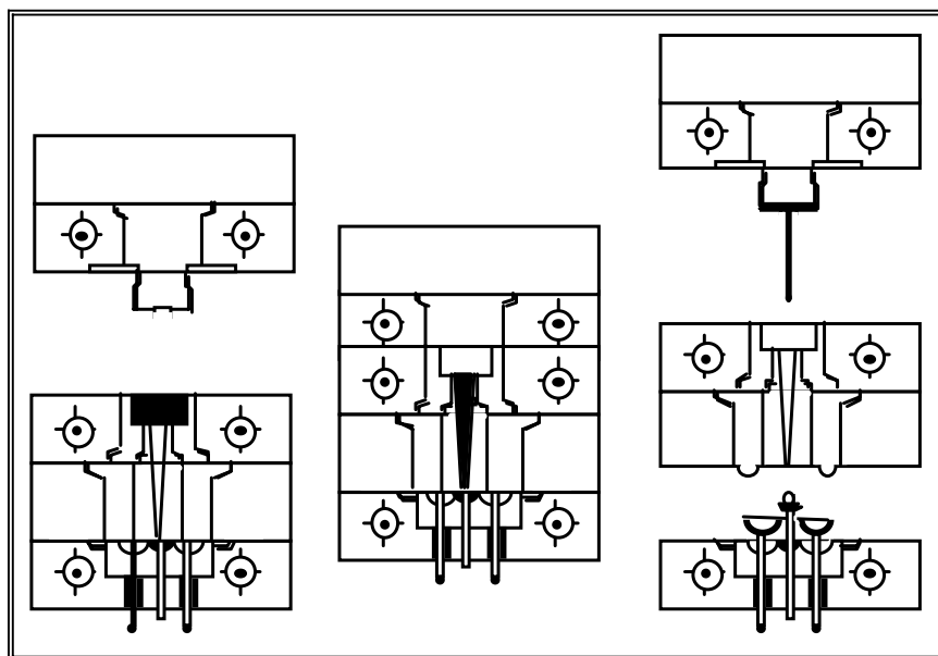
Figure 11: Transfer Molding
