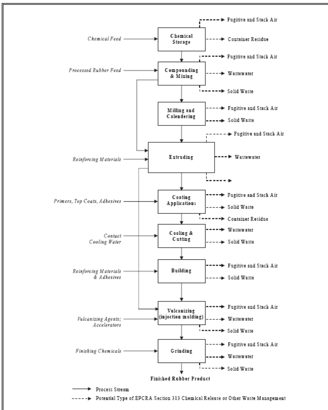
Figure 13: Rubber Manufacturing Process
