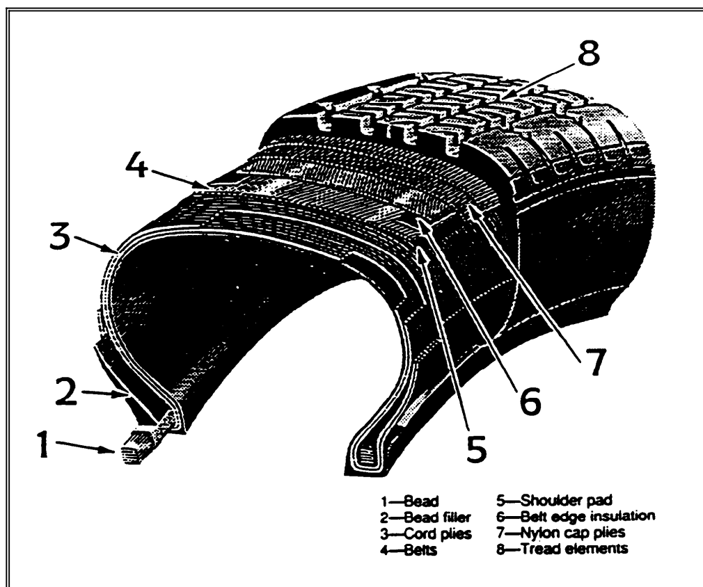
Figure 16: Tire Formation
