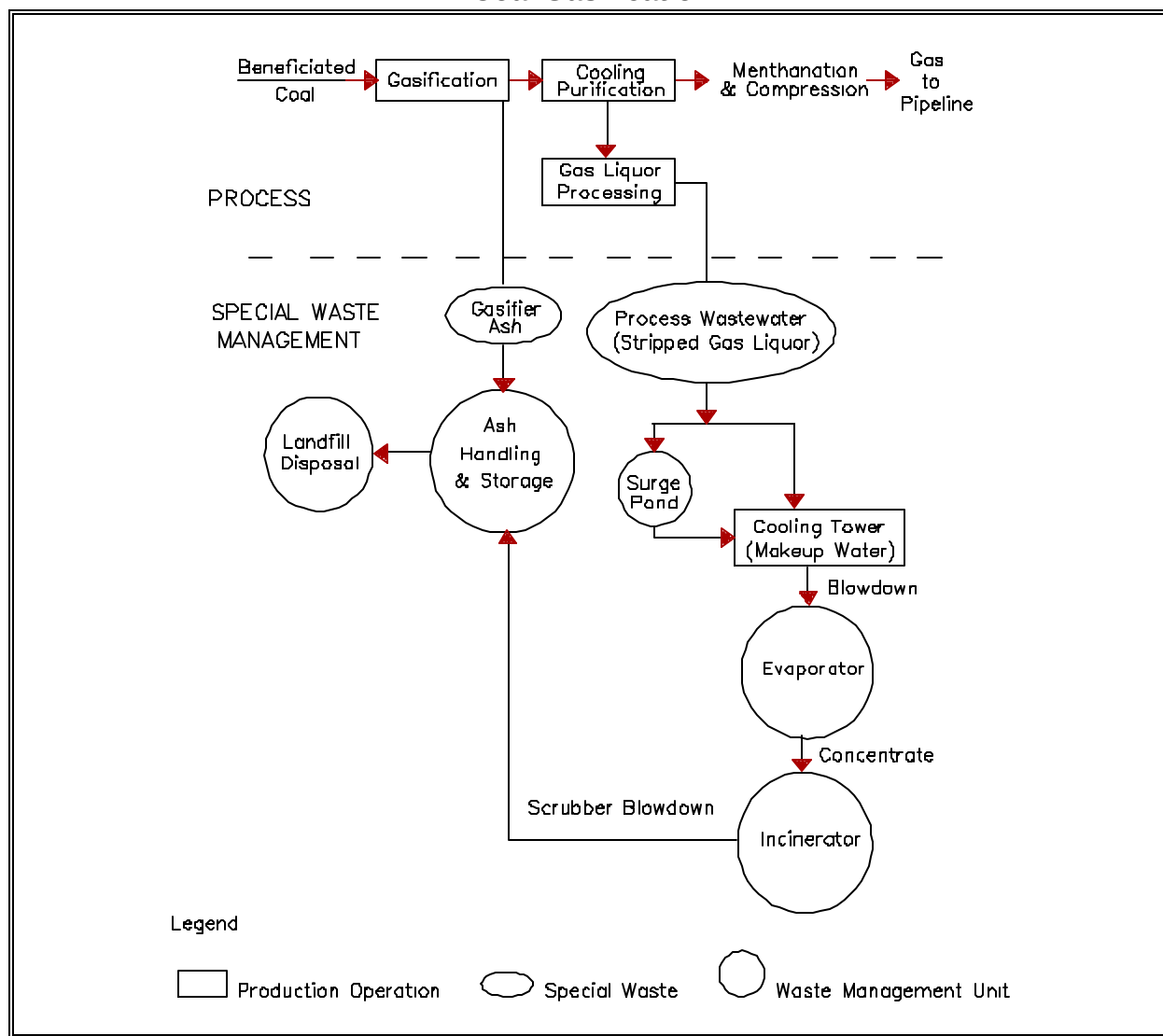
Exhibit 5-1 Coal Gasification
