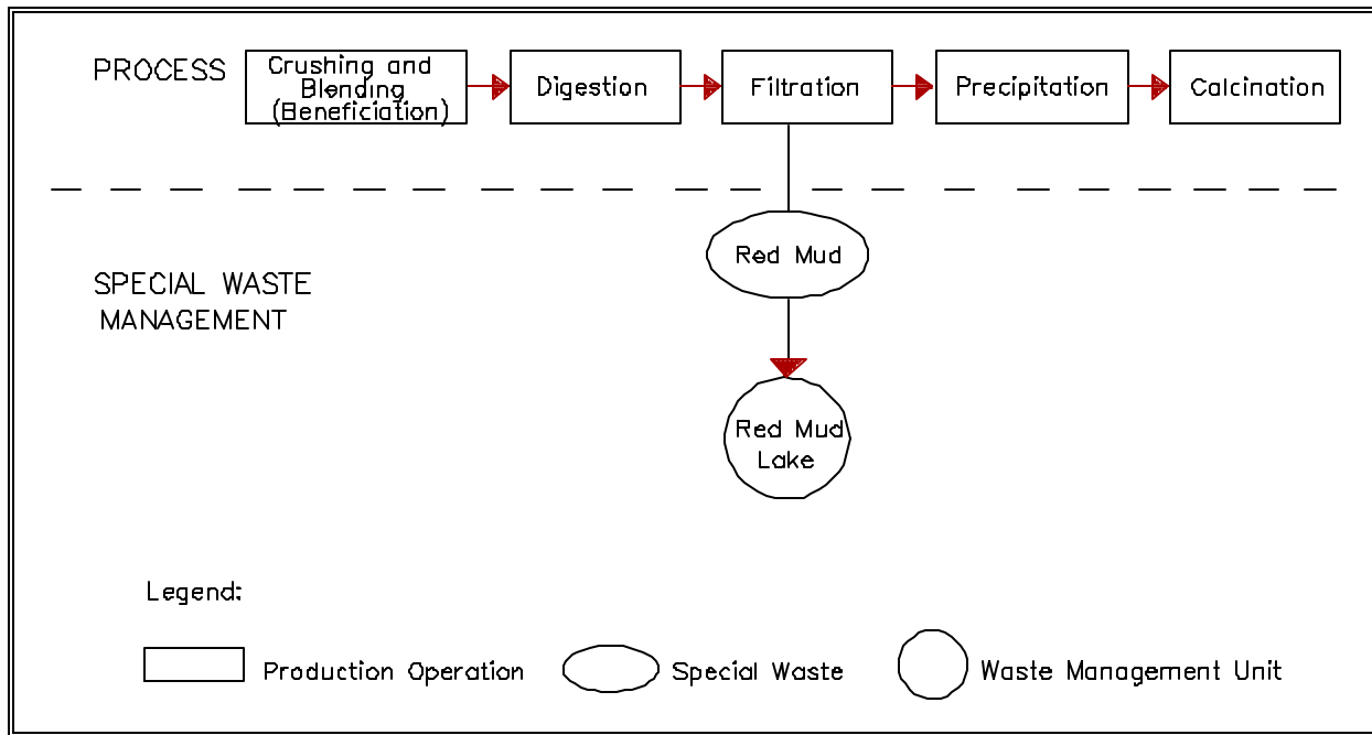
Exhibit 3-2 Alumina Production
