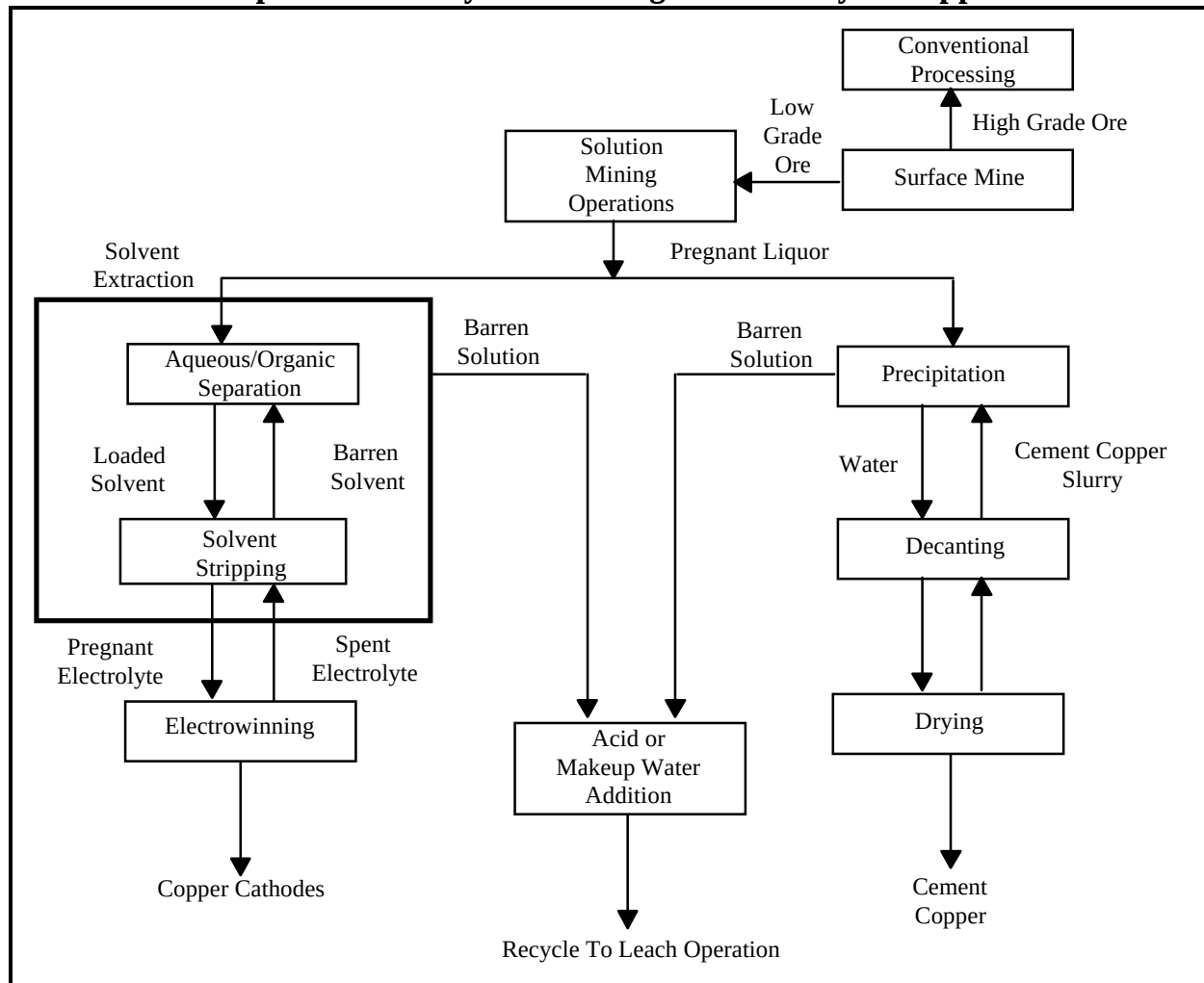
Exhibit 11 Representative Hydrometallurgical Recovery of Copper
