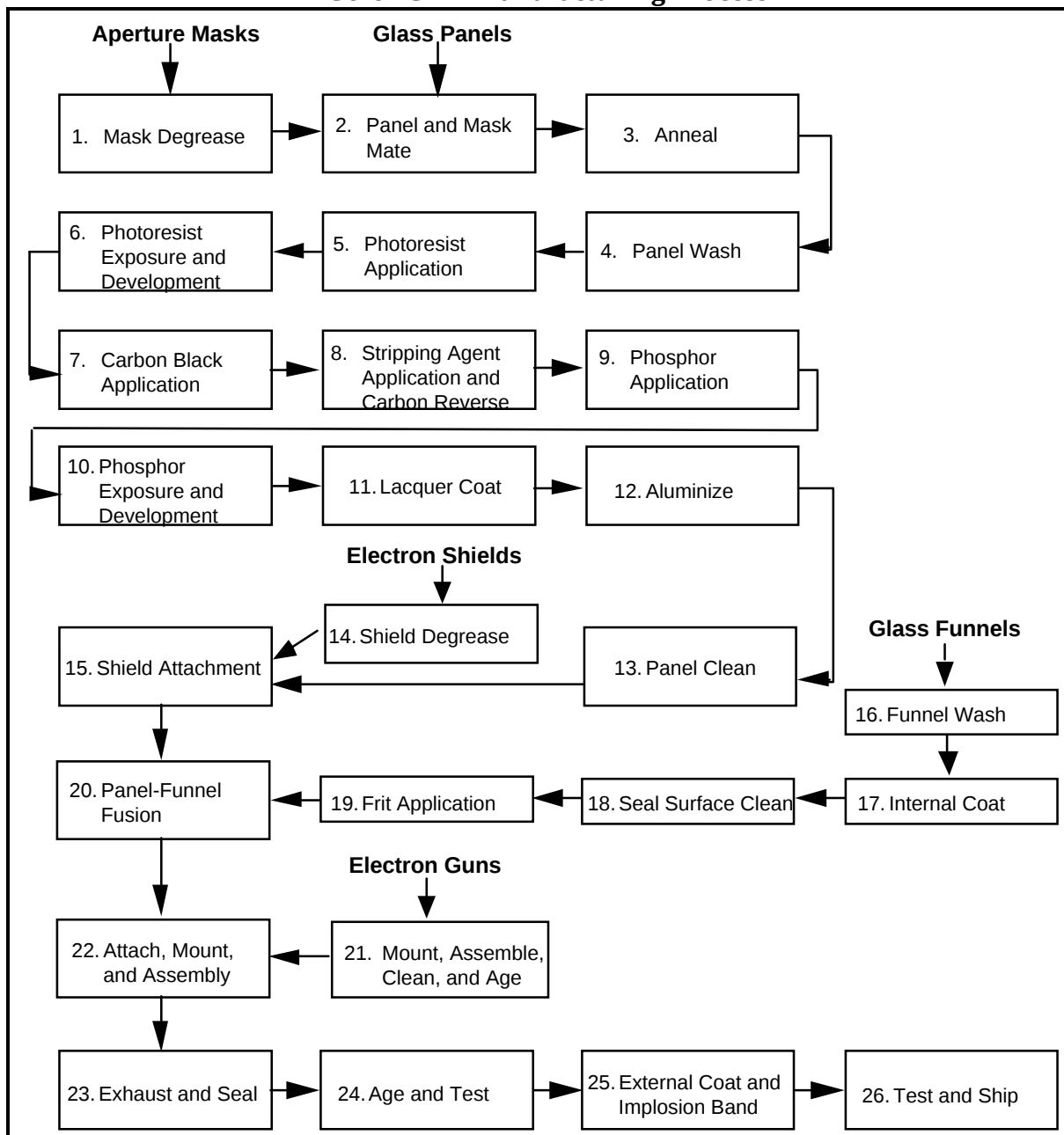
Exhibit 13 Color CRT Manufacturing Process
