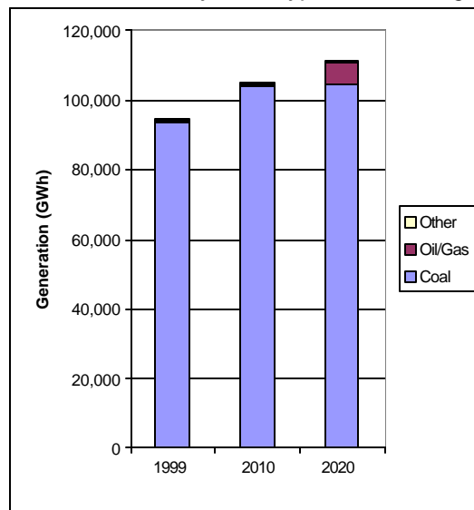
Figure 3. Current and Projected Generation by Fuel Type in West Virginia under Clear Skies (GWh) 9
