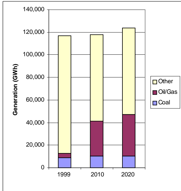
Current and Projected Generation by Fuel Type in Washington under Clear Skies (GWh)
