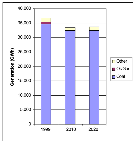
Current and Projected Generation by Fuel Type in Utah under Clear Skies (GWh)
