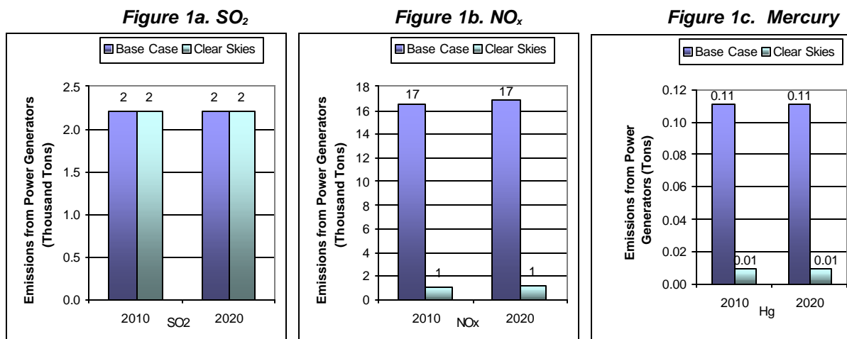
Figures 1a, 1b and 1c. Existing Clean Air Act Regulations (base case 4 ) vs. Clear Skies South Dakota in 2010 and 2020
