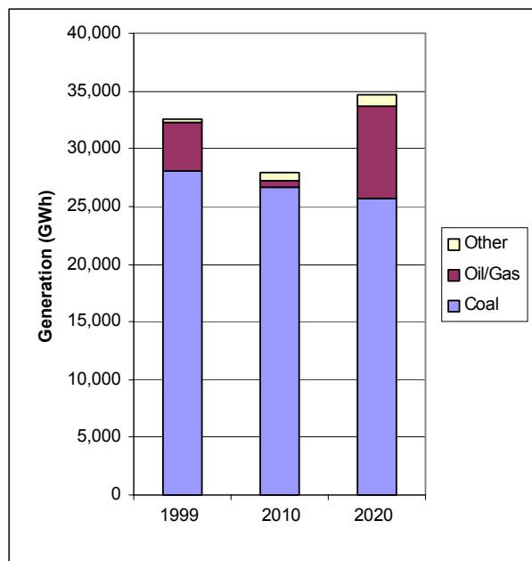
Current and Projected Generation by Fuel Type in New Mexico under Clear Skies (GWh)
