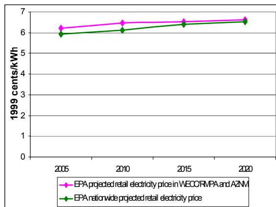
Projected National Retail Electricity Prices and Prices in New Mexico under Clear Skies (2005-2020)
