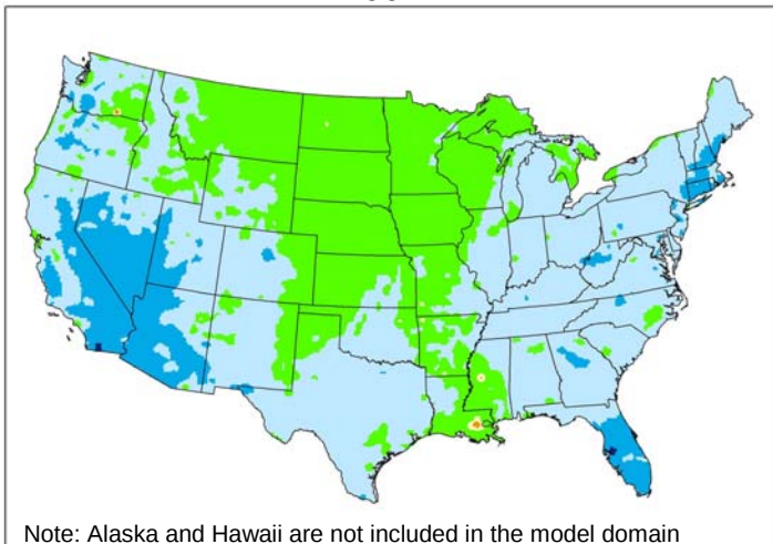
Projected Changes in Nitrogen Deposition with the Base Case in 2020 Compared to 2001
