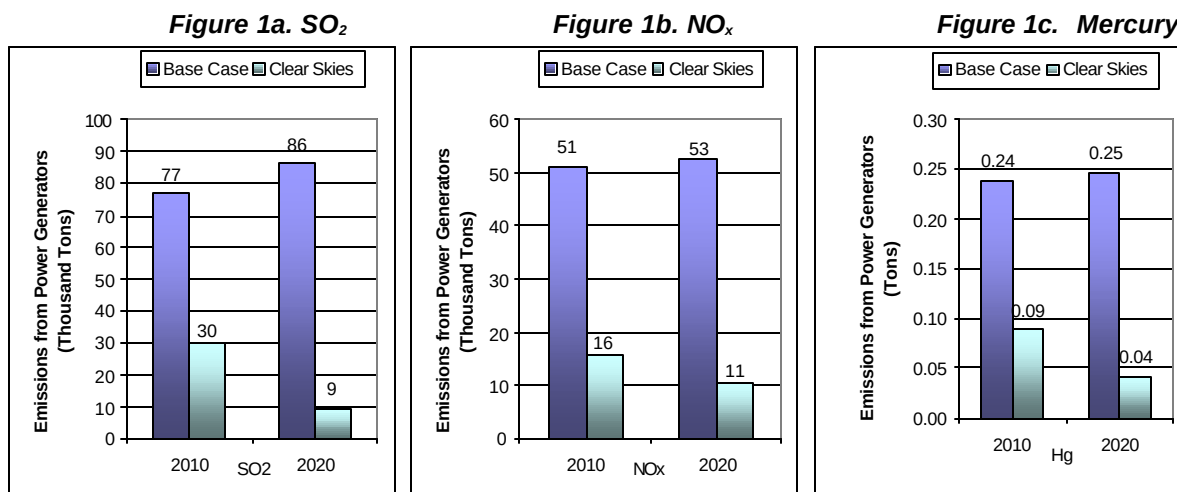
Figures 1a, 1b and 1c. Existing Clean Air Act Regulations (base case 5 ) vs. Clear Skies in Mississippi in 2010 and 2020
