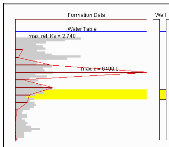
Figure 7 Estimated borehole concentration of 995 µg/L for a ten-foot long well screen placed 70 feet below the land surface.
