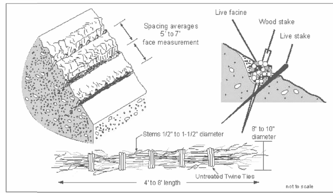
SOIL BIOENGINEERING - LIVE FASCINES RIVERFRONT
