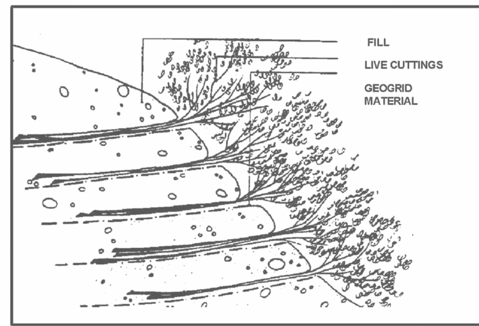
BIOTECHNICAL STABILIZATION - GEOGRIDS WITH BRUSHLAYER RIVERFRONT
