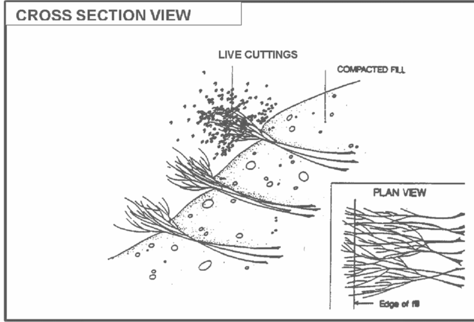
SOIL BIOENGINEERING - BRUSHLAYER RIVERFRONT
