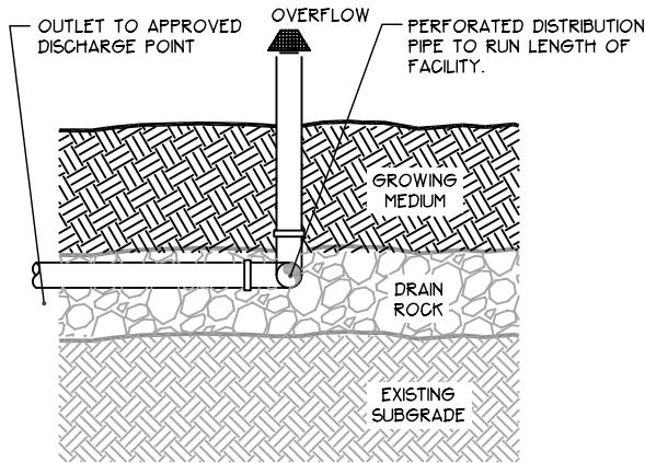
PARTIAL INFILTRATION
