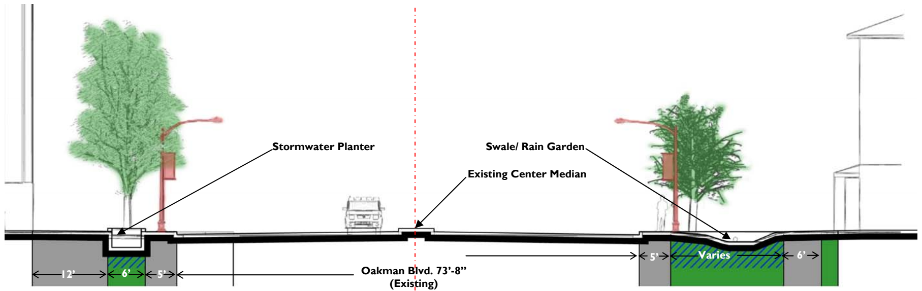
Section C-C
