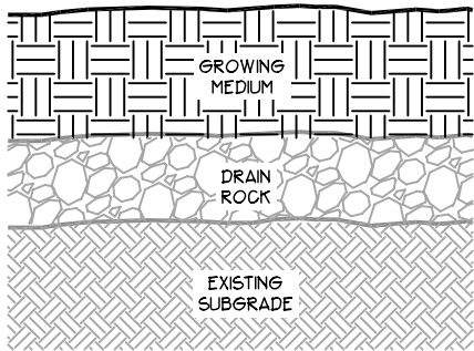
INFILTRATION
