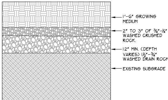
SOIL PROFILE
