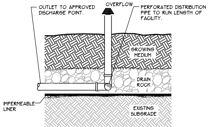
FLOW-THROUGH
