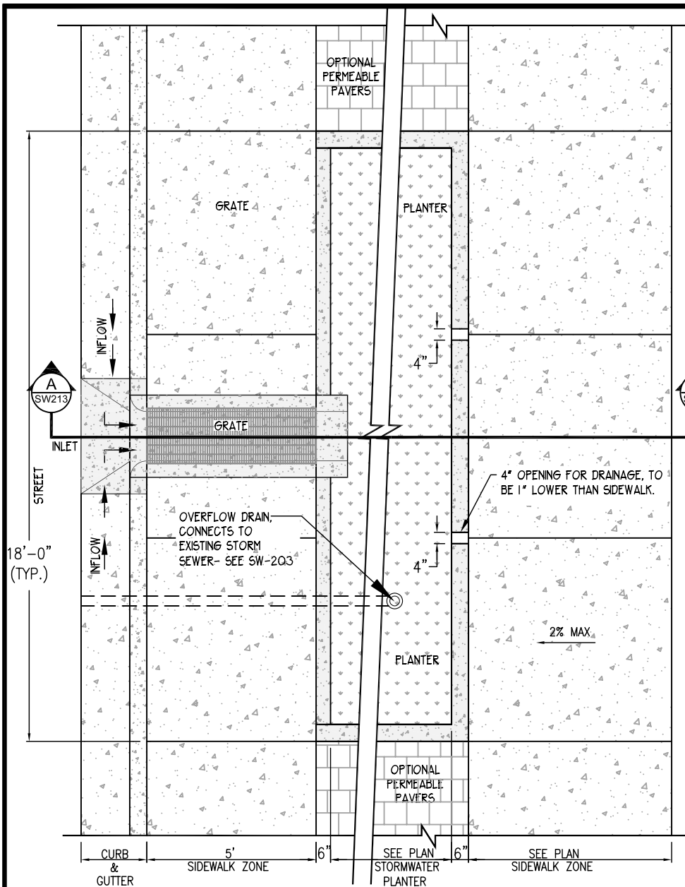
PLANTER PLAN
