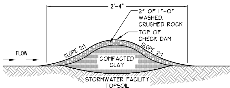
CHECK DAM
