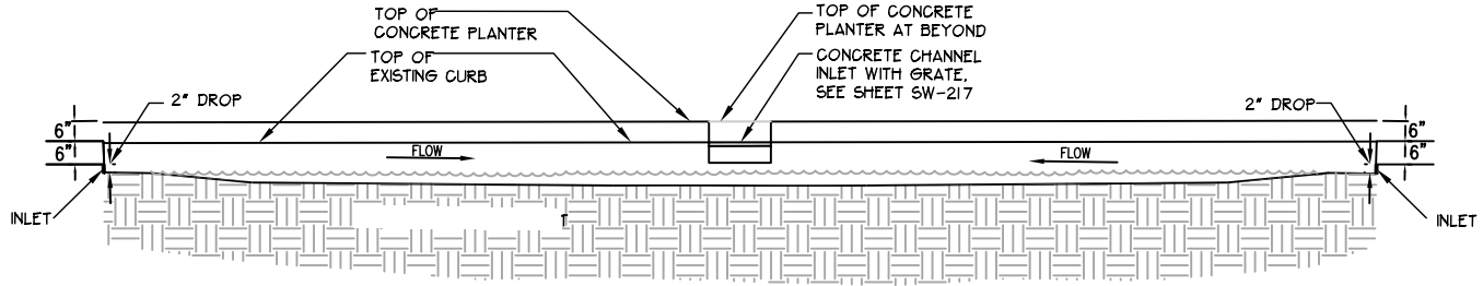
SECTION B-B CURB EXTENSION PROFILE
