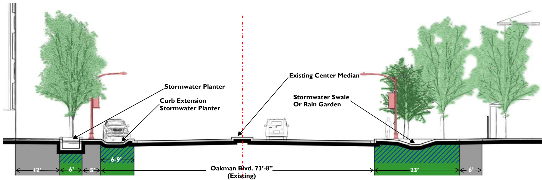
Section B-B
