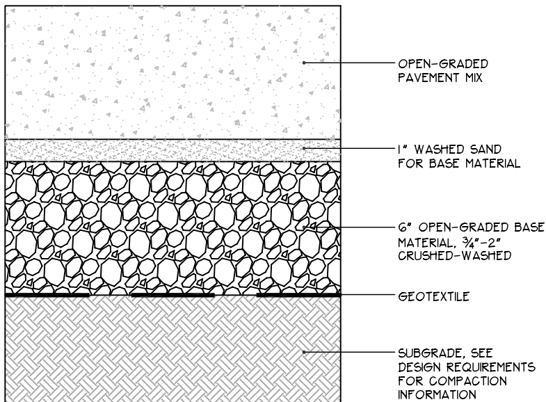
PERVIOUS (OPEN GRADED) CONCRETE AND ASPHALT SYSTEMS
