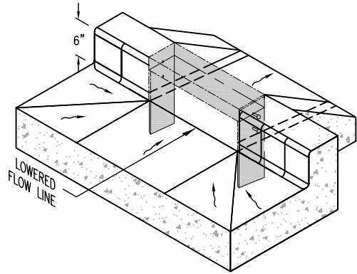
ISOMETRIC
