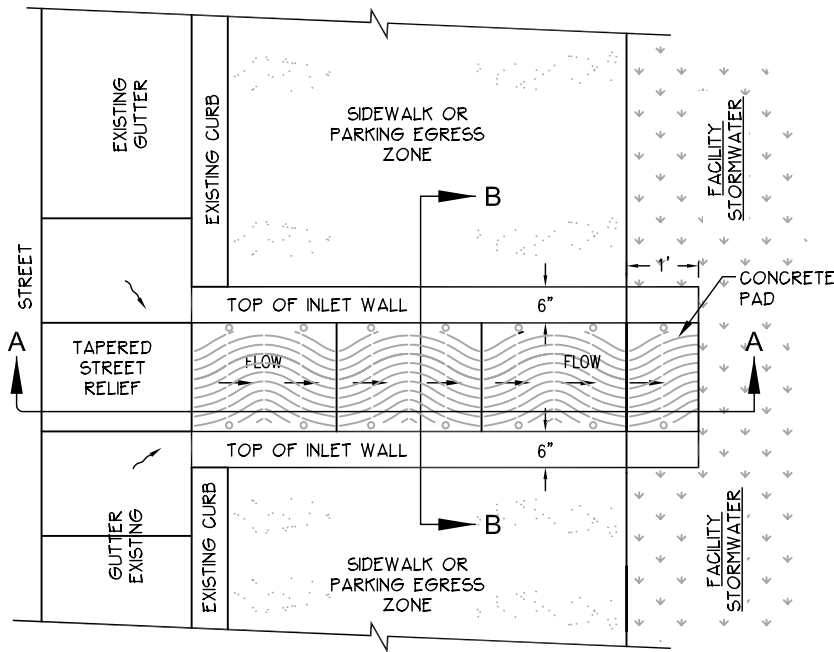
PLAN VIEW
