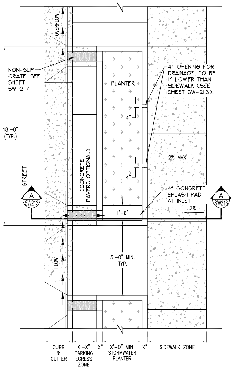
PLANTER PLAN
