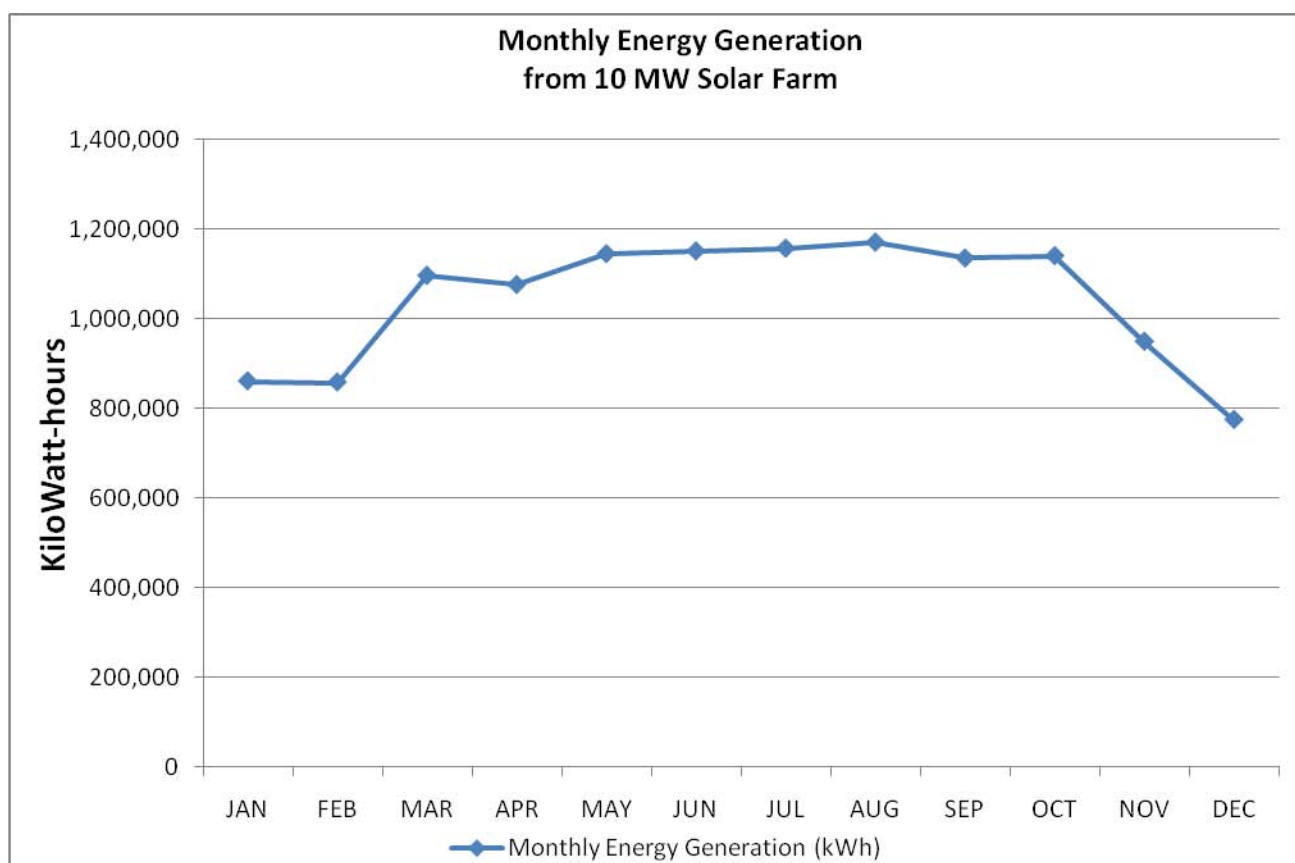
Figure 5. Monthly Energy Generation from 10 MW Solar Farm
