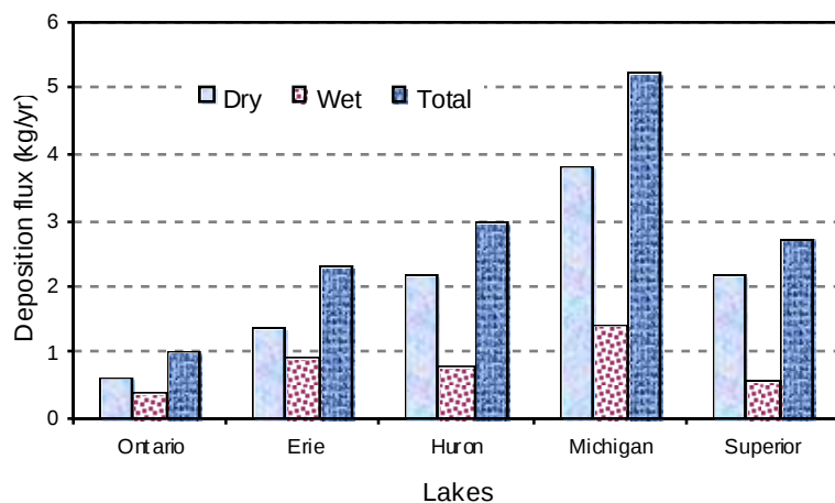
Figure 1. Modeled annual HCB loadings ( \text{kg yr}^{-1} ) to the Great Lakes in 2000 due to dry, wet, and total (dry + wet) deposition.
