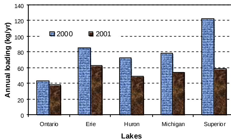
Figure 2. Annual total net gas exchange fluxes ( \text{kg yr}^{-1} ) of HCB in the five lakes.
