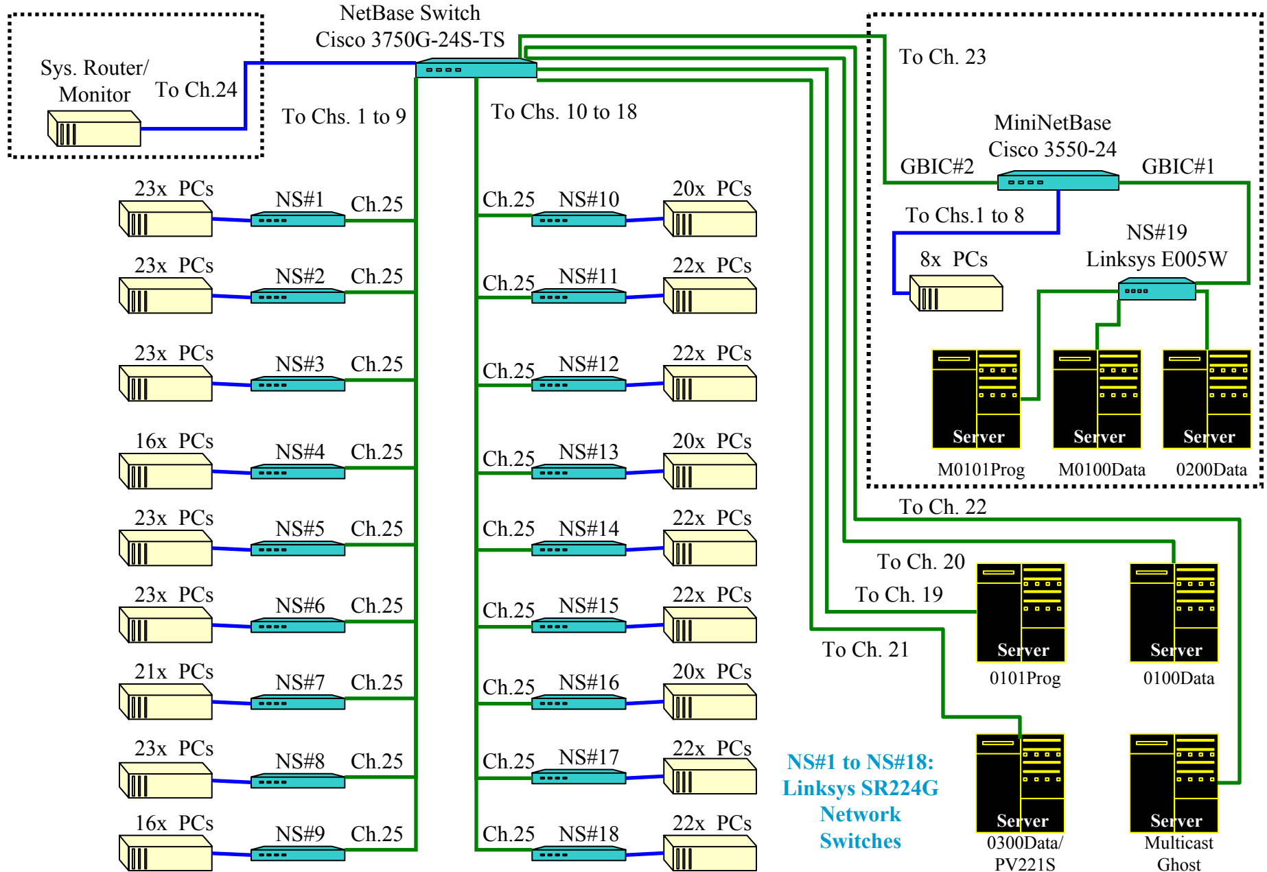
Figure 3A: SuperMUSE Master Network Switch Wiring Details
