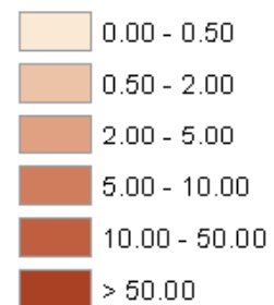
2008 (SF2) PM 2.5 (tons/SqMi)
