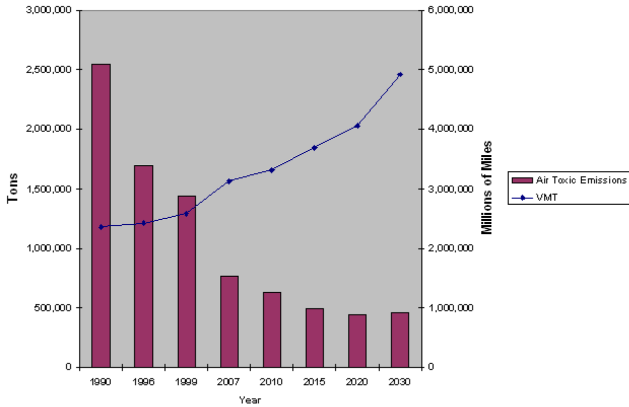
Highway Vehicle Air Toxic Emissions vs. Vehicle Miles Travelled (VMT)
