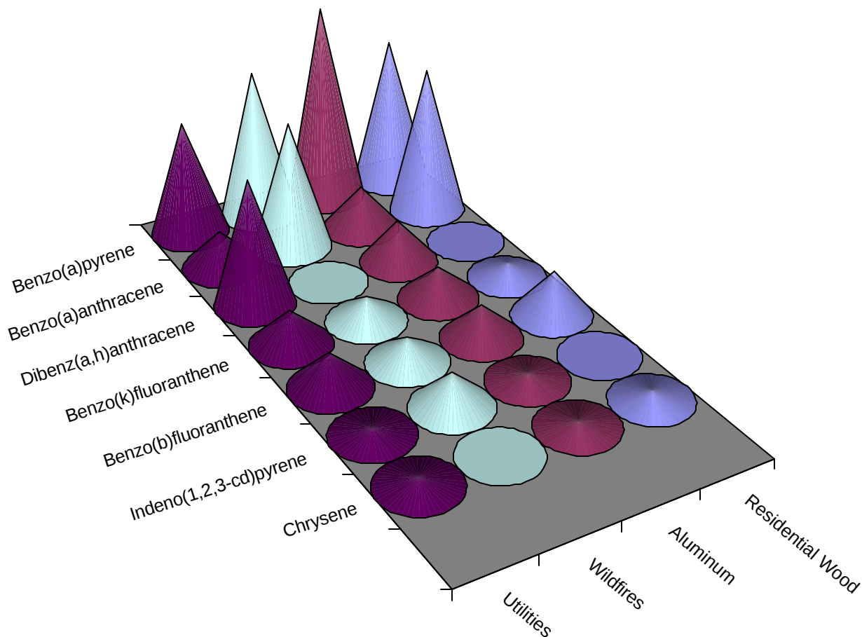
Figure 1. Distribution of BaP equivalence among 7 carcinogenic PAHs emitted from 4 large POM sources
