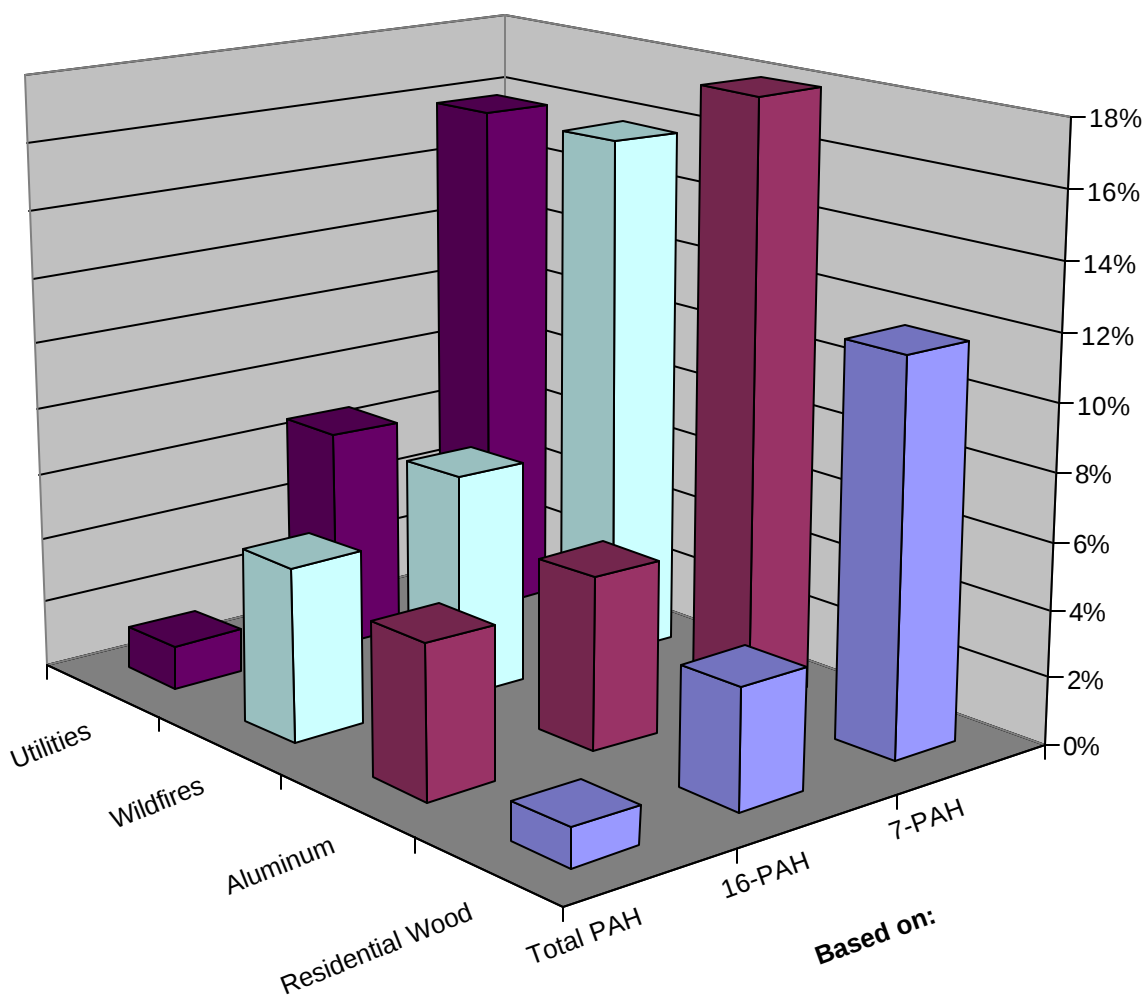
Figure 2. Benzo[a]pyrene equivalence for four large POM sources
