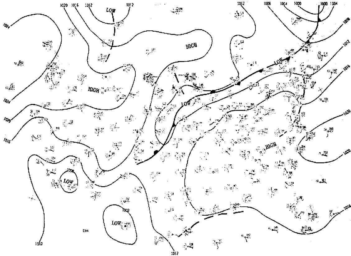
Figure 3.5-1 Daily Weather Maps for July 14, 1995
