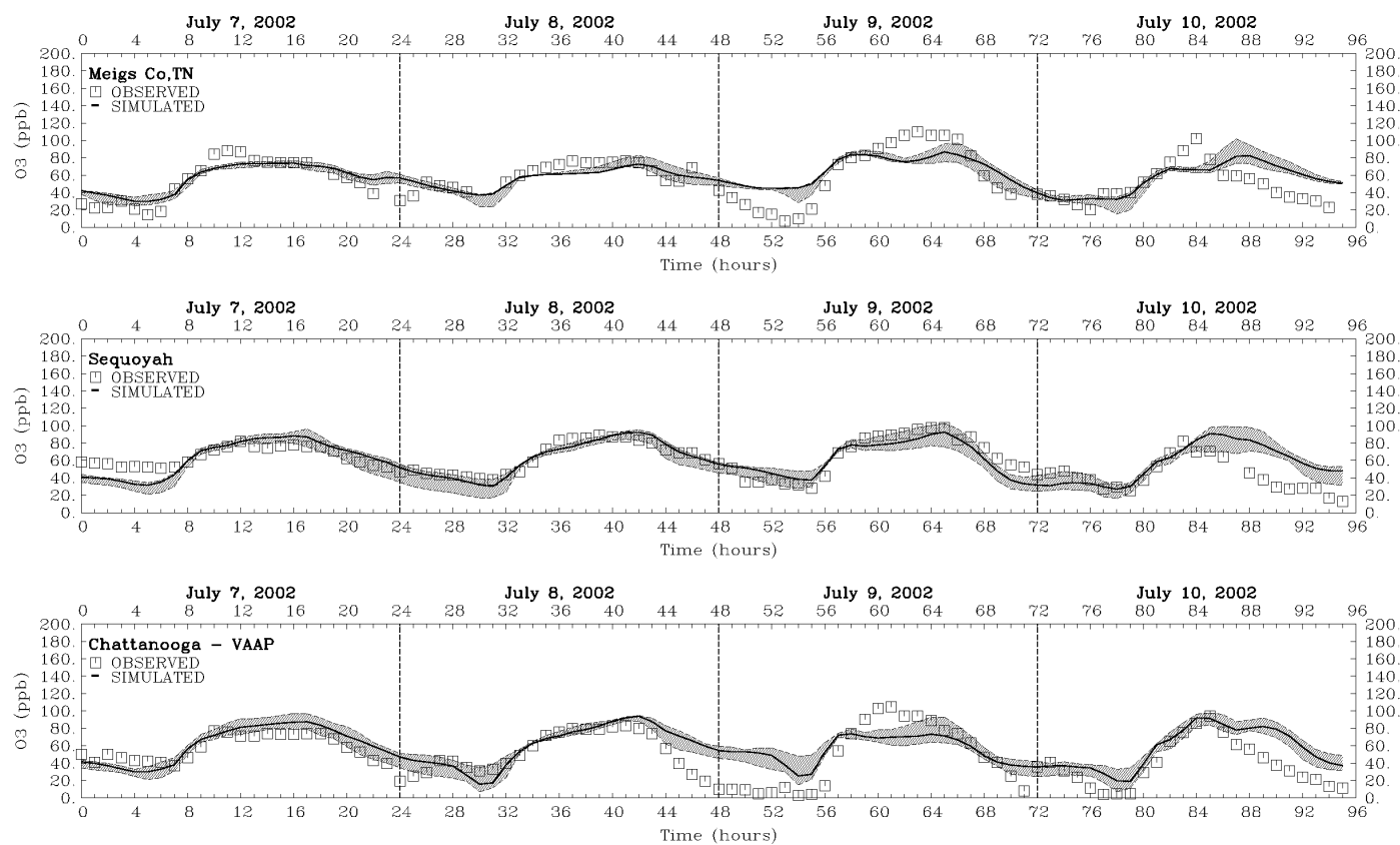
Figure 6-11l. 2001 Episode Time Series: Chattanooga EAC Area, July 7-10, 2002
