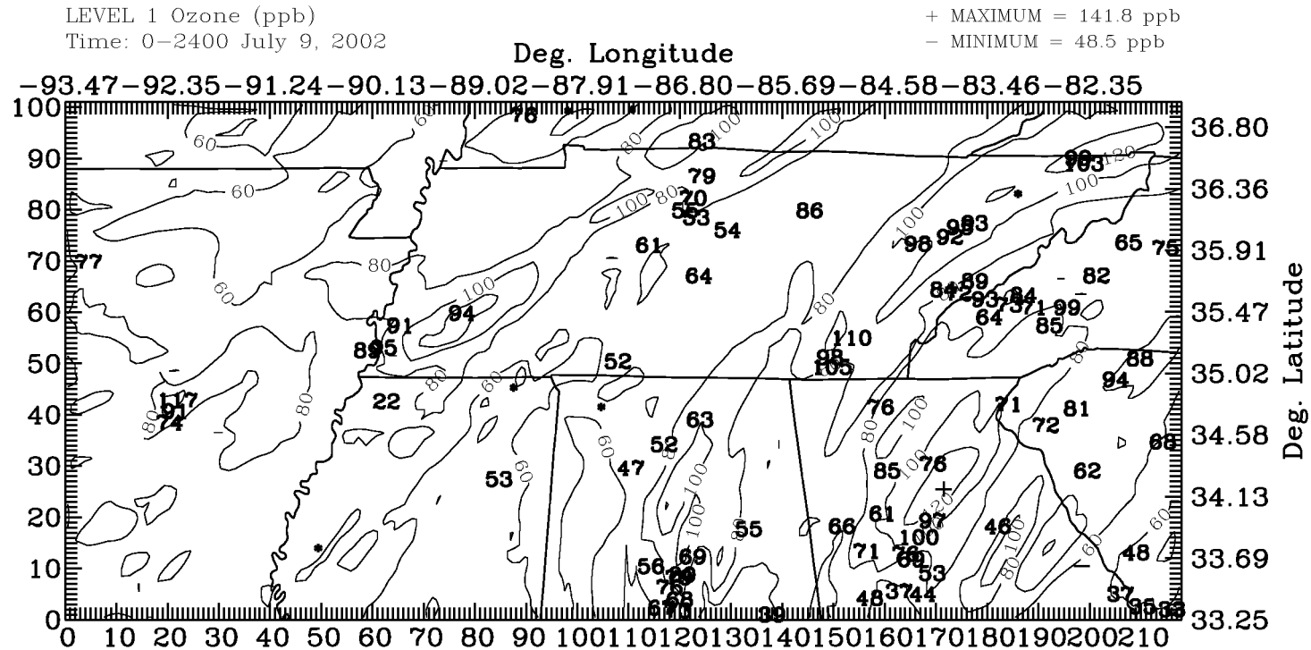
Figure 6-10f. Daily Maximum 1-Hour Ozone, Grid 3, July 9, 2002
