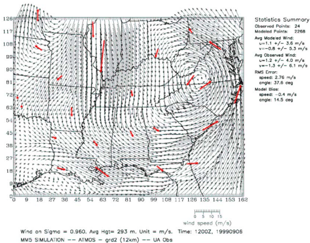
Figure 4-1i. MM5-Derived 12-km Wind Field for 0700 EST on 6 September 1999 at Approximately 300 m agl.
