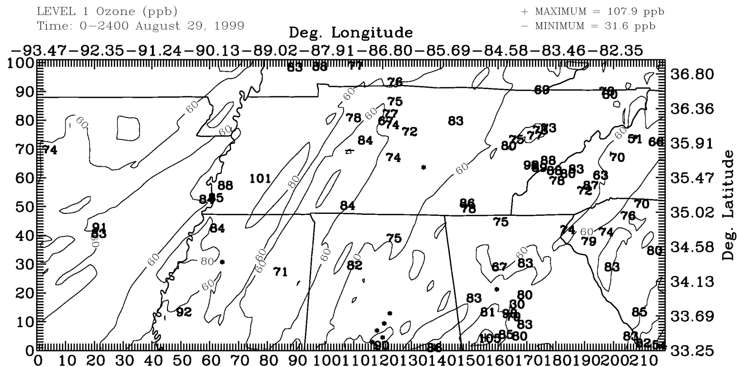
Figure 6-2a. Daily Maximum 1-Hour Ozone, Grid 3, August 29, 1999
