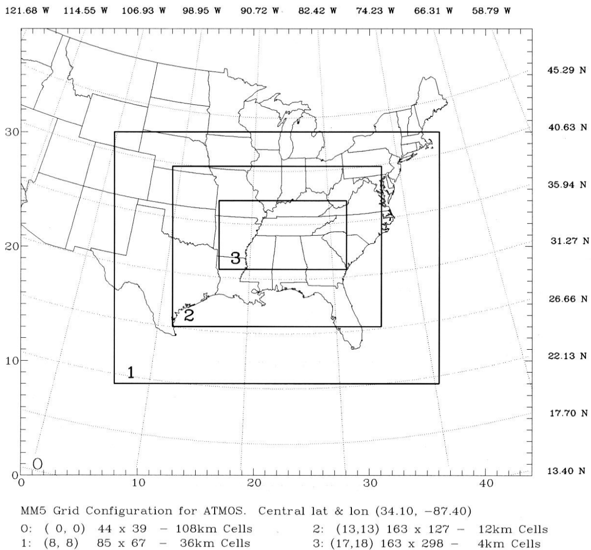
Figure 1-4. MM5 Modeling Domain for the ATMOS Application
