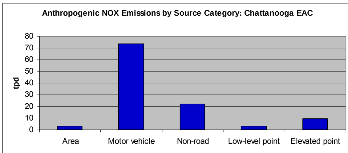
Figure 1-13d. Weekday Anthropogenic Emissions (tpd) in the Chattanooga EAC Area by Species and Source Category
