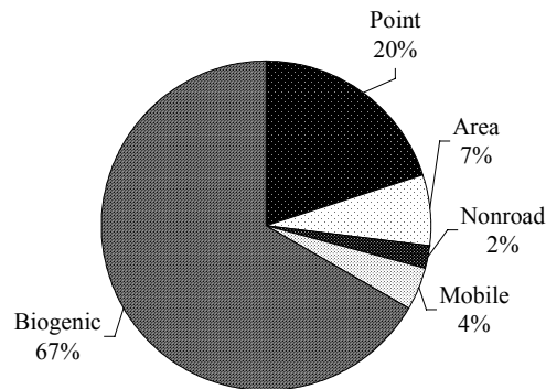
Figure 4.4-4: 2007 Unifour Area VOC Emissions by Source
