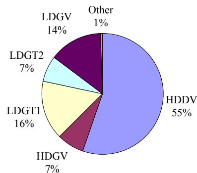
Figure 4.4-6: 2007 Unifour Area Highway Mobile NO x Sources
