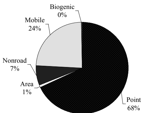
Figure 4.4-1: 2000 Unifour Area NOx Emissions by Source
