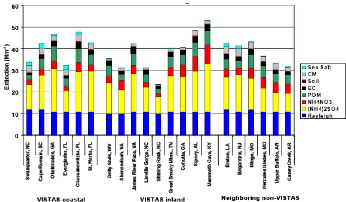
Figure 1.8 - Average light extinction for the 20% Clearest Days in 2000-2004 at VISTAS and neighboring Class I areas using new IMPROVE equation
