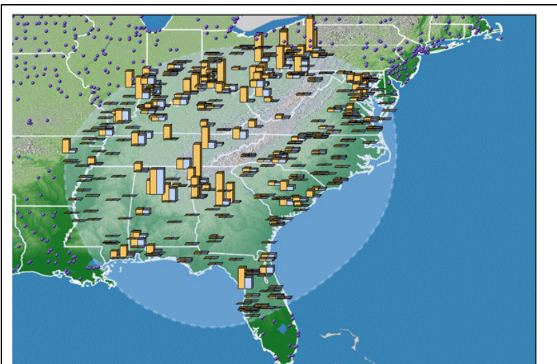
Projected SO 2 Emissions from Existing Power Generation Sources in the Southern Blue Ridge Airshed in 2020
