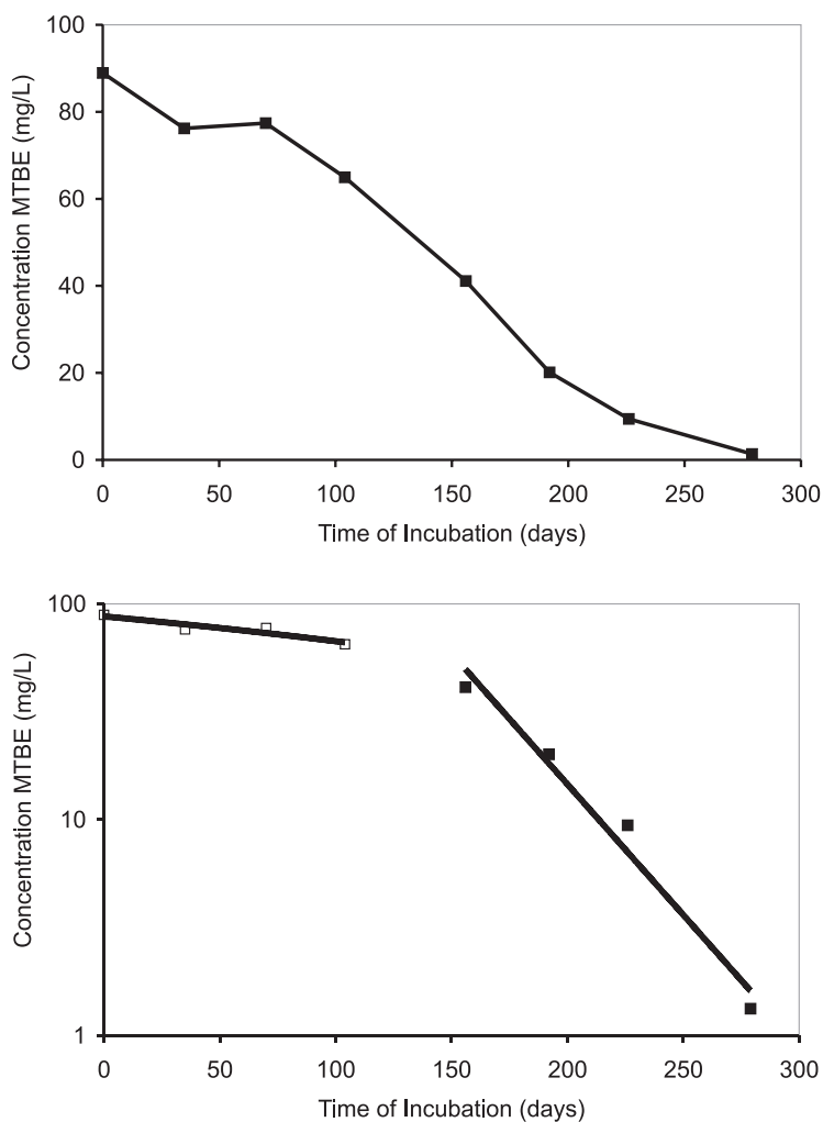
Figure 4.5 -Anaerobic biodegradation of MTBE at high concentration in an enrichment culture constructed with sediment from the microcosms used to produce the data in Figure 4.4. The same data are plotted on an arithmetic scale in the upper panel and a logarithmic scale in the lower panel.
