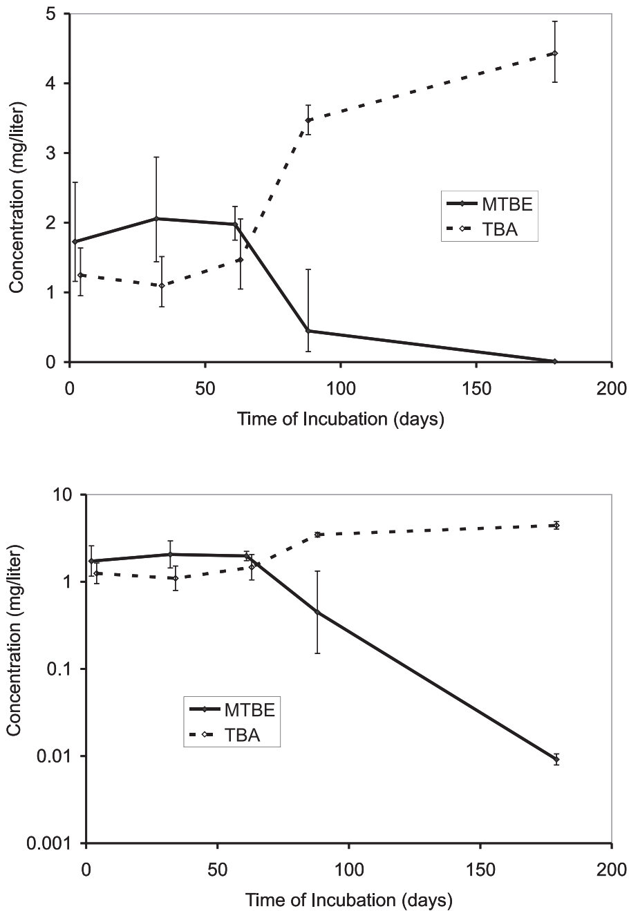
Figure 4.4 -Anaerobic biodegradation of MTBE and production of TBA in microcosms constructed with sediment from a gasoline spill site. The error bars are the 95% confidence intervals on the geometric mean concentration. The same data are plotted on an arithmetic scale in the upper panel and a logarithmic scale in the lower panel.
