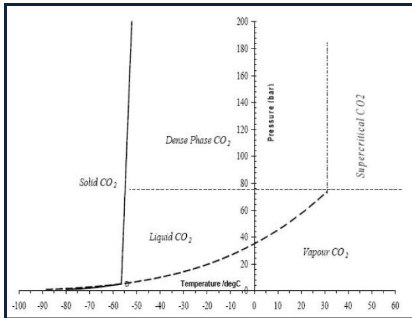
Figure 2. Pure Carbon dioxide phase diagram
