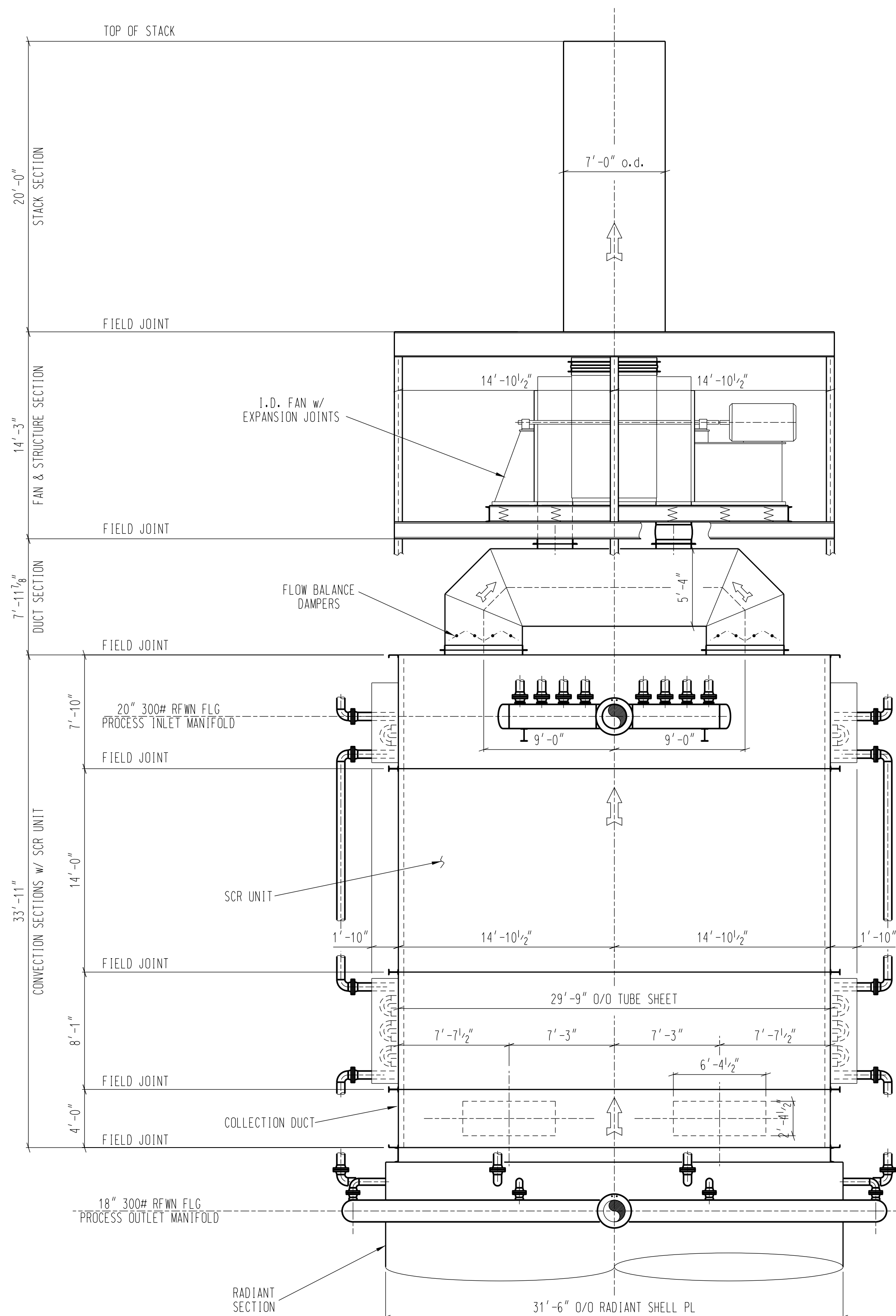
SIDEWALL ELEVATION VIEW
