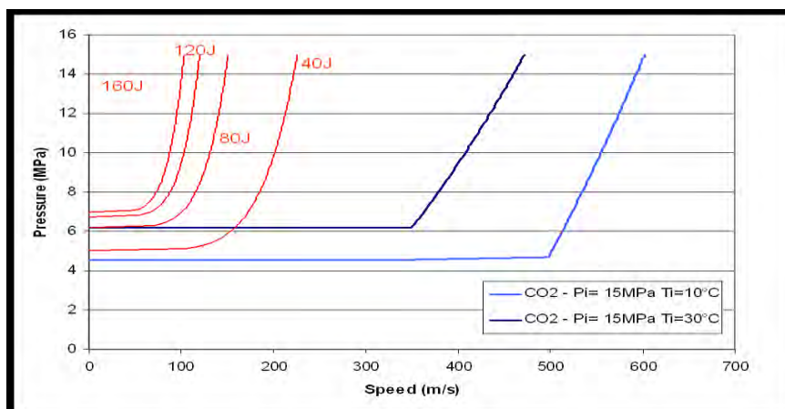
Figure 7: Arrest / propagation for a CO 2 pipelines on the base of Battelle model coupled with the decompression model of CSM, GASMISC
