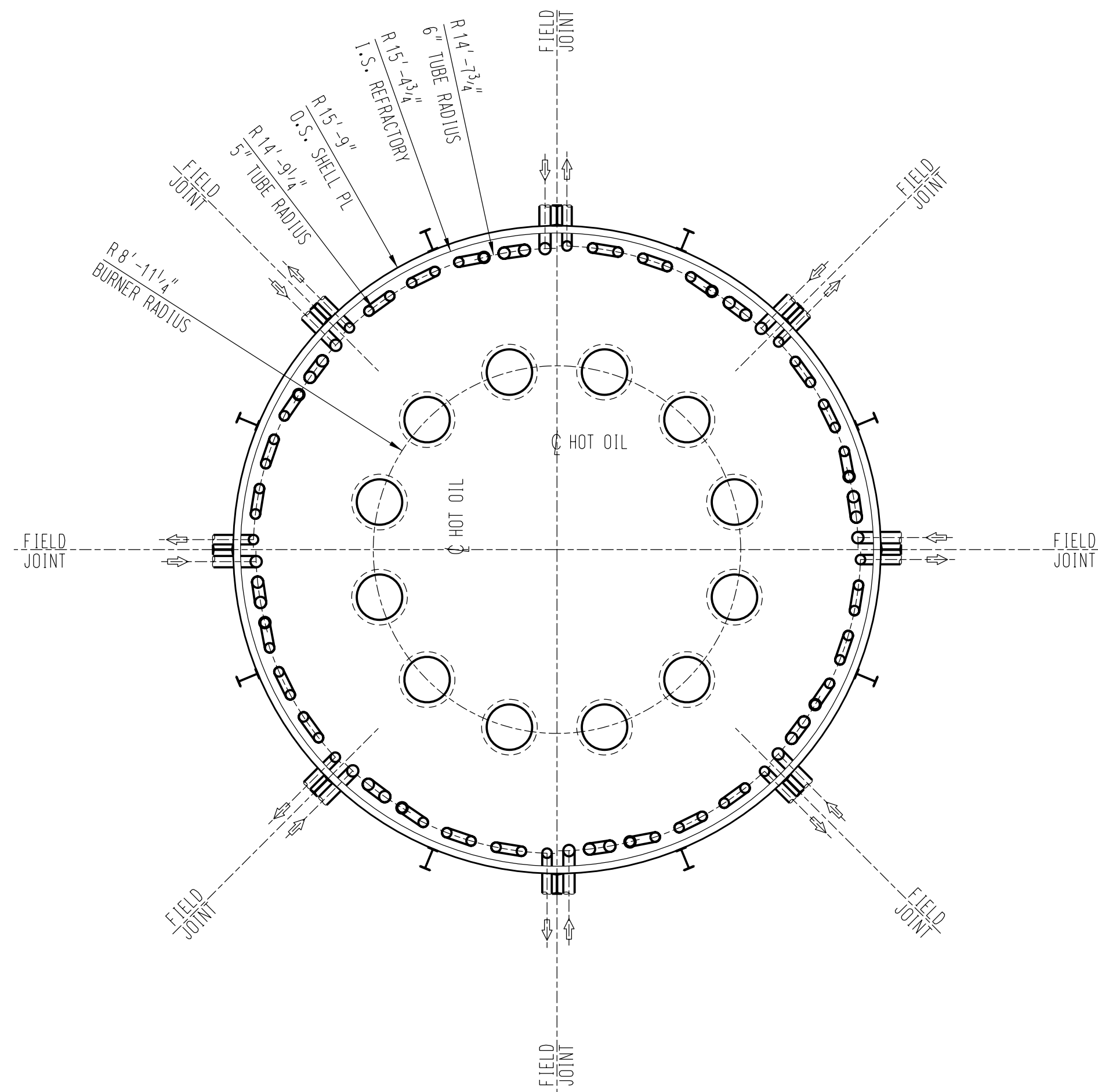
PLAN VIEW @ RADIANT TUBES, BURNERS, & FLOOR
