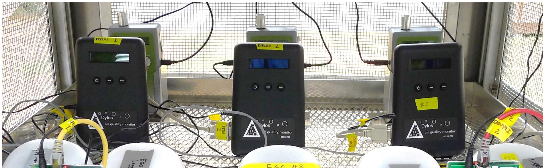
Figure A-3. Dylos units inside the chamber (Figure A-1) during field deployment.
