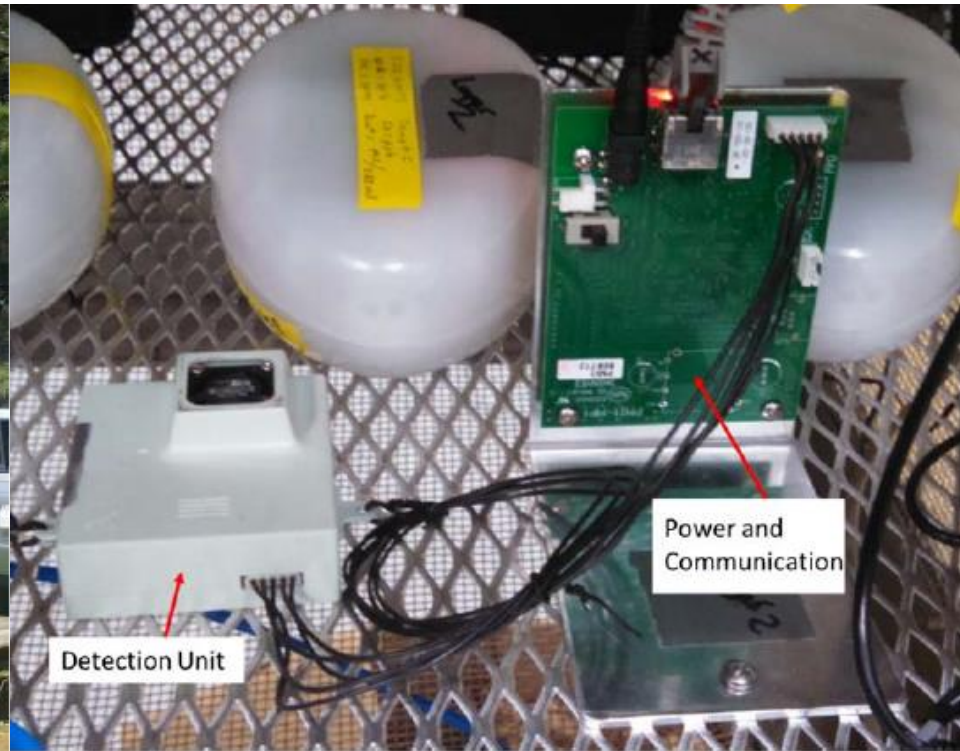
Figure A-2. Shinyei detection and power/communication units inside the chamber (Figure A-1) during field deployment.
