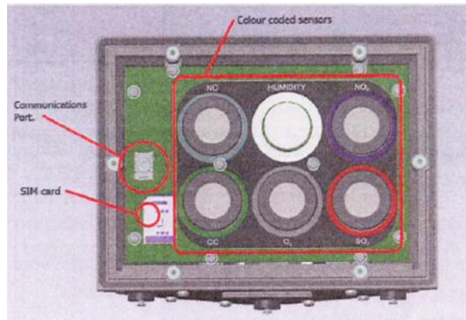
Figure A-12. Underside of the AQ Mesh unit showing the included sensors, the communication port, and the SIM card.
