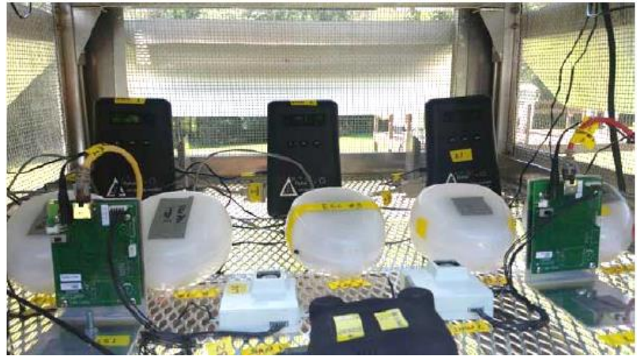
Figure A-14. Air Quality Egg inside the chamber (Figure A-1) during field deployment.
