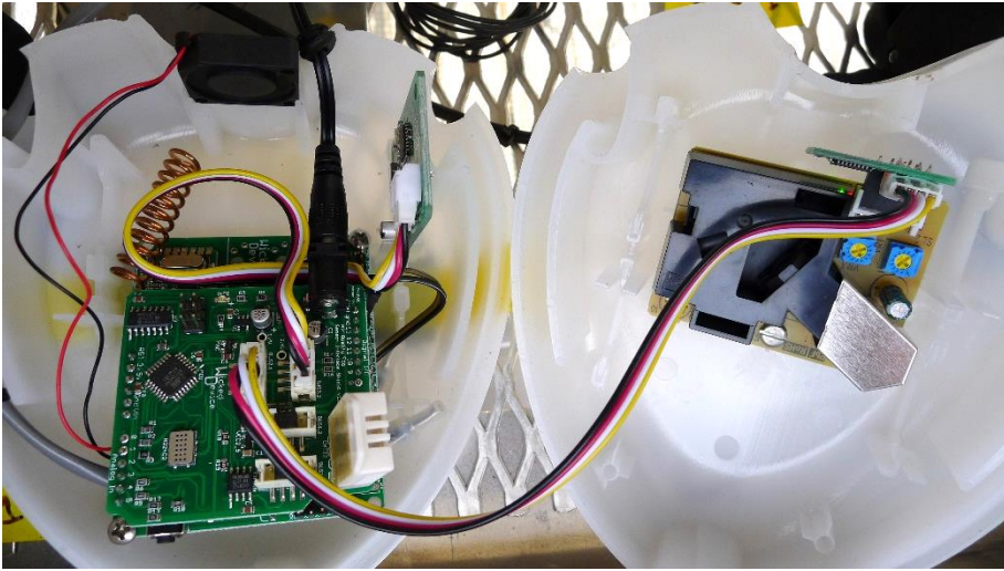
Figure A-13. Inside of Air Quality Egg.
