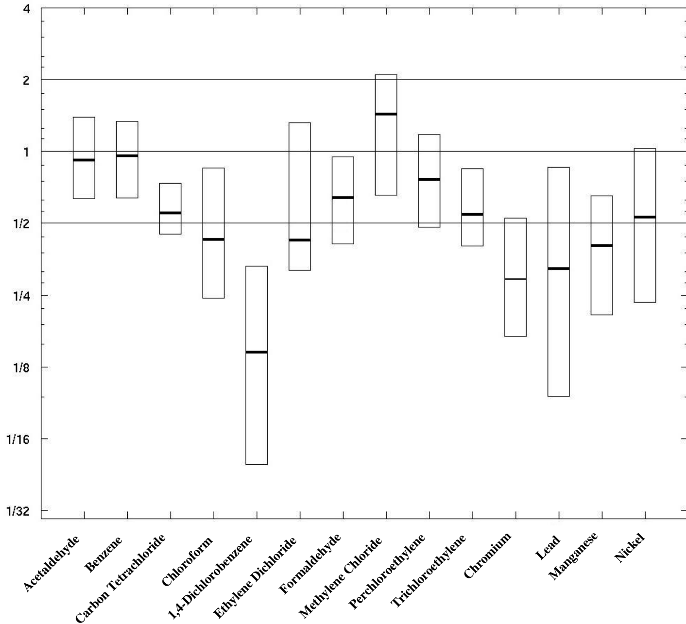
Figure 1. Ratio box plot showing distribution of 1999 model/monitor ratios for each pollutant. The bottom of each box is the 25th percentile, the top is the 75th percentile, and the horizontal line in the middle is the median. See the number of sites summarized in each box plot (see Table1).
